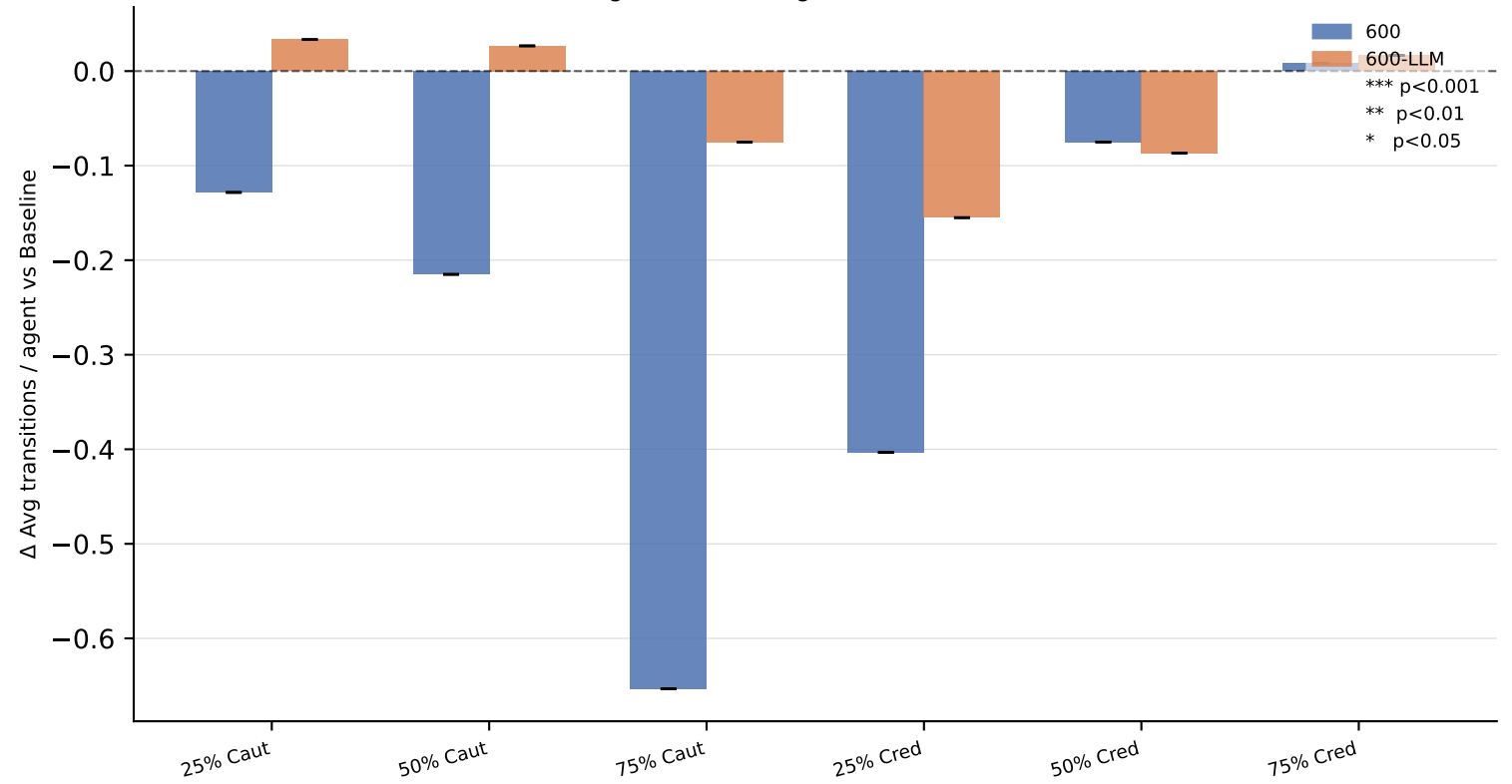
\Delta vs Baseline — Avg transitions / agent — thread 524990163446140928
