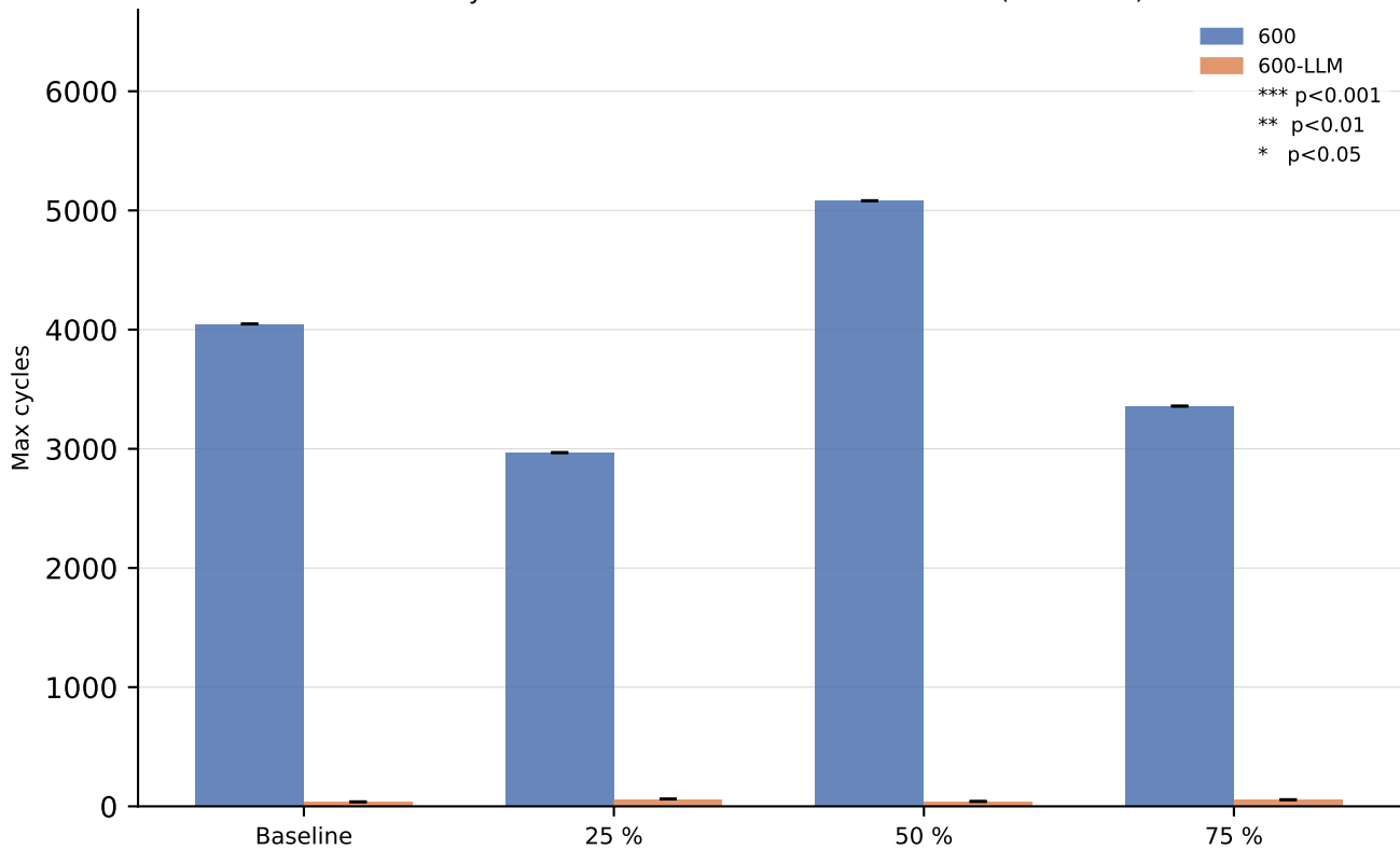
Max cycles — thread 524990163446140928 (credulous)
