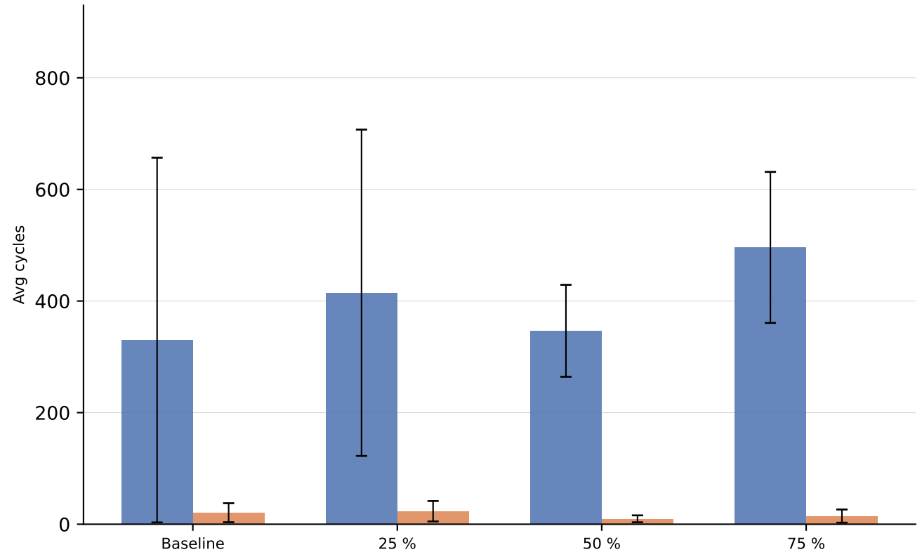
Avg cycles — all threads (cautious)
