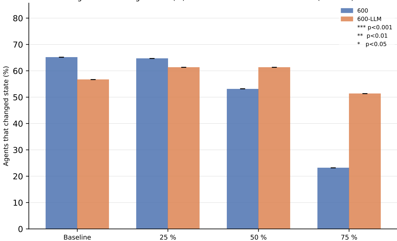
Agents that changed state (%) — thread 524990163446140928 (cautious)
