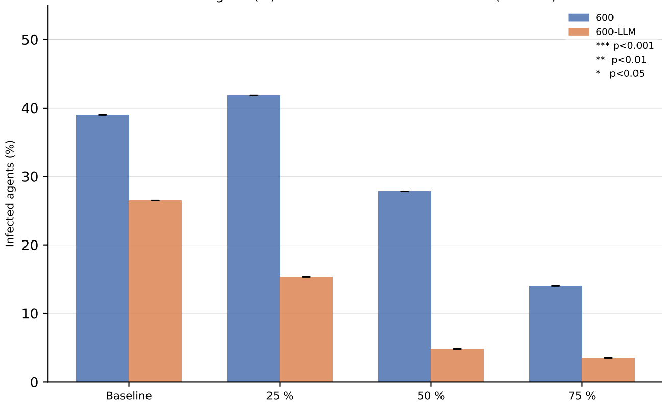
Infected agents (%) — thread 524990163446140928 (cautious)
