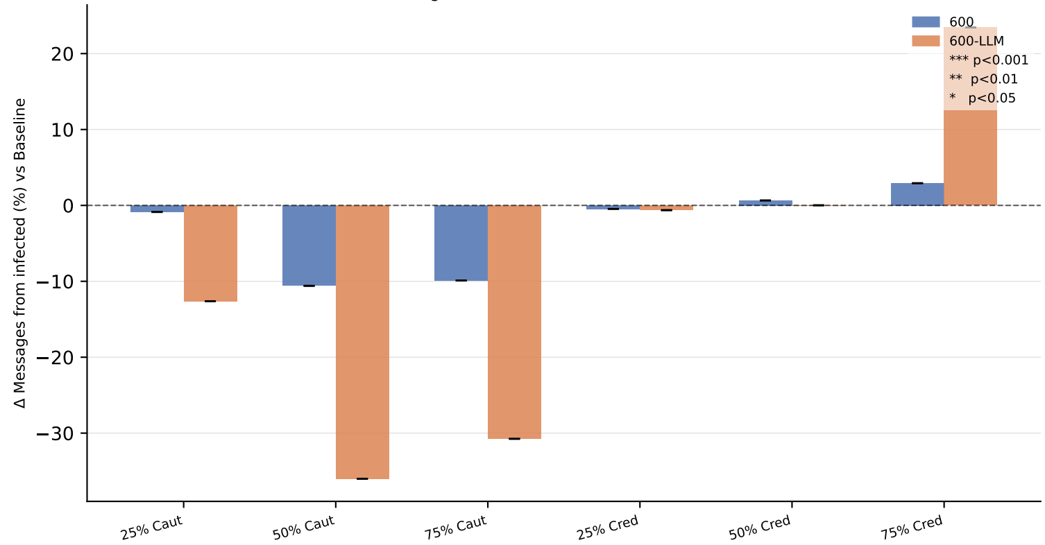
Δ vs Baseline — Messages from infected (%) — thread 524949443607412737
