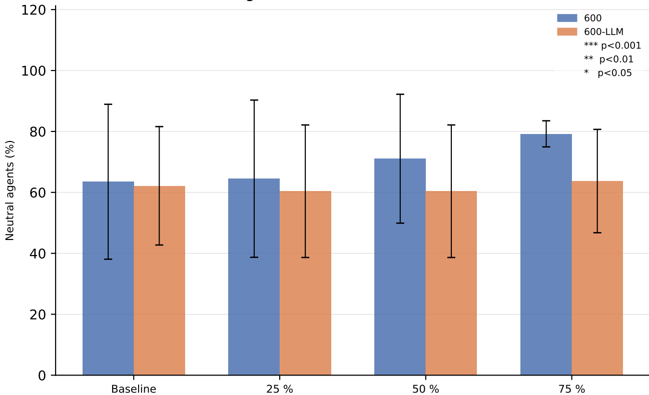
Neutral agents (%) — all threads (cautious)
