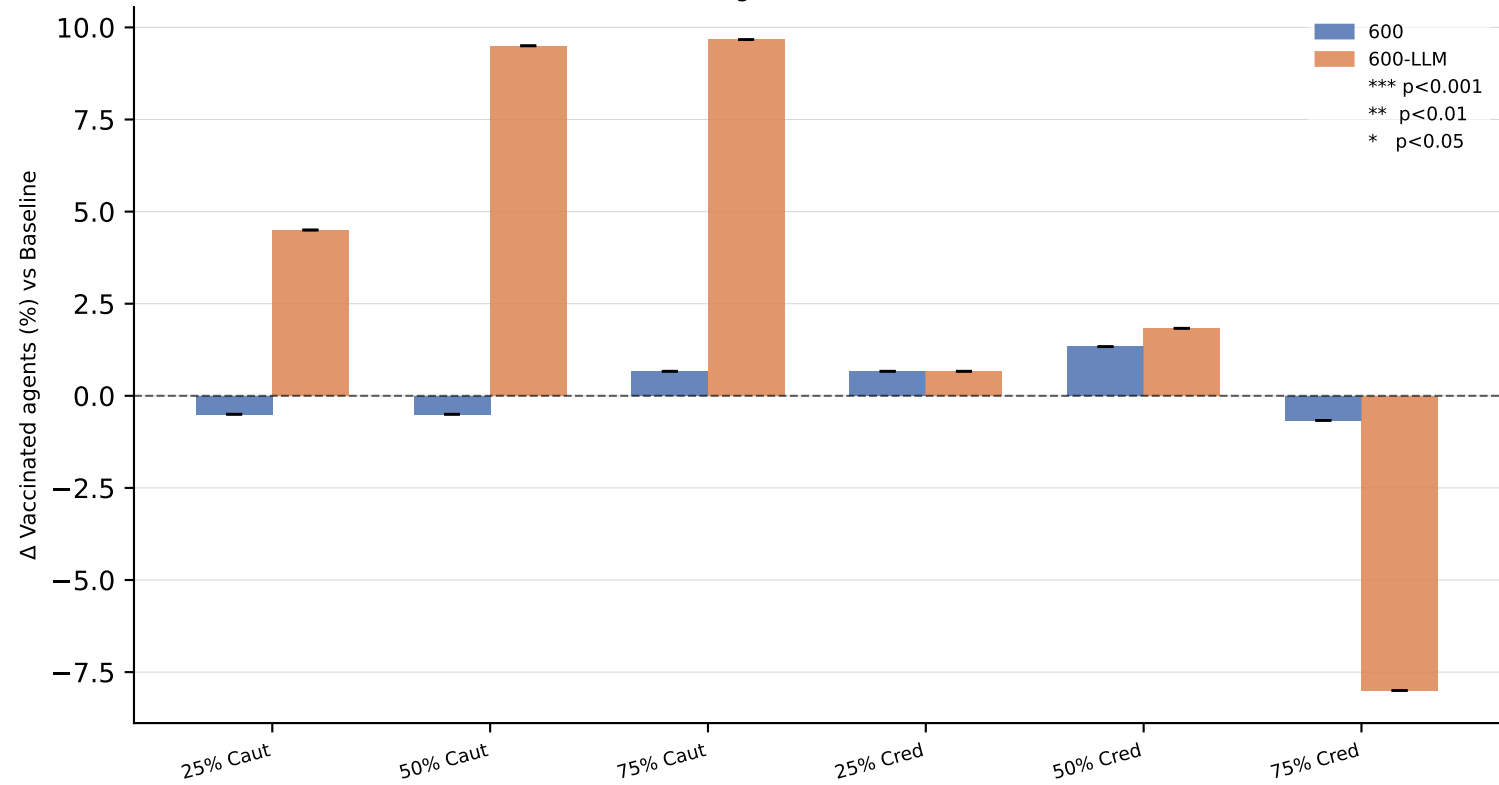
Δ vs Baseline — Vaccinated agents (%) — thread 524949443607412737
