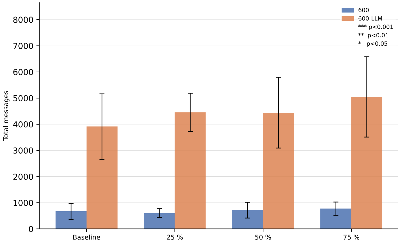
Total messages — all threads (credulous)
