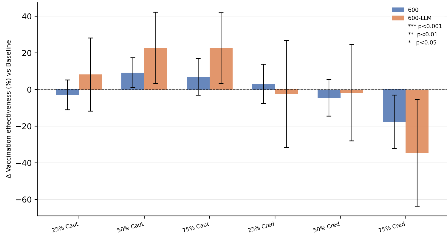
\Delta vs Baseline — Vaccination effectiveness (%) — all threads
