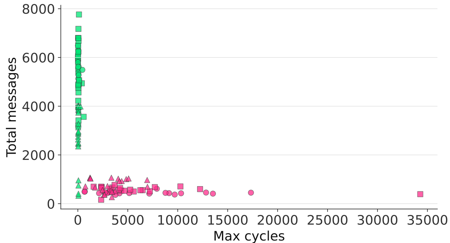
Total messages vs max cycles (per run)
