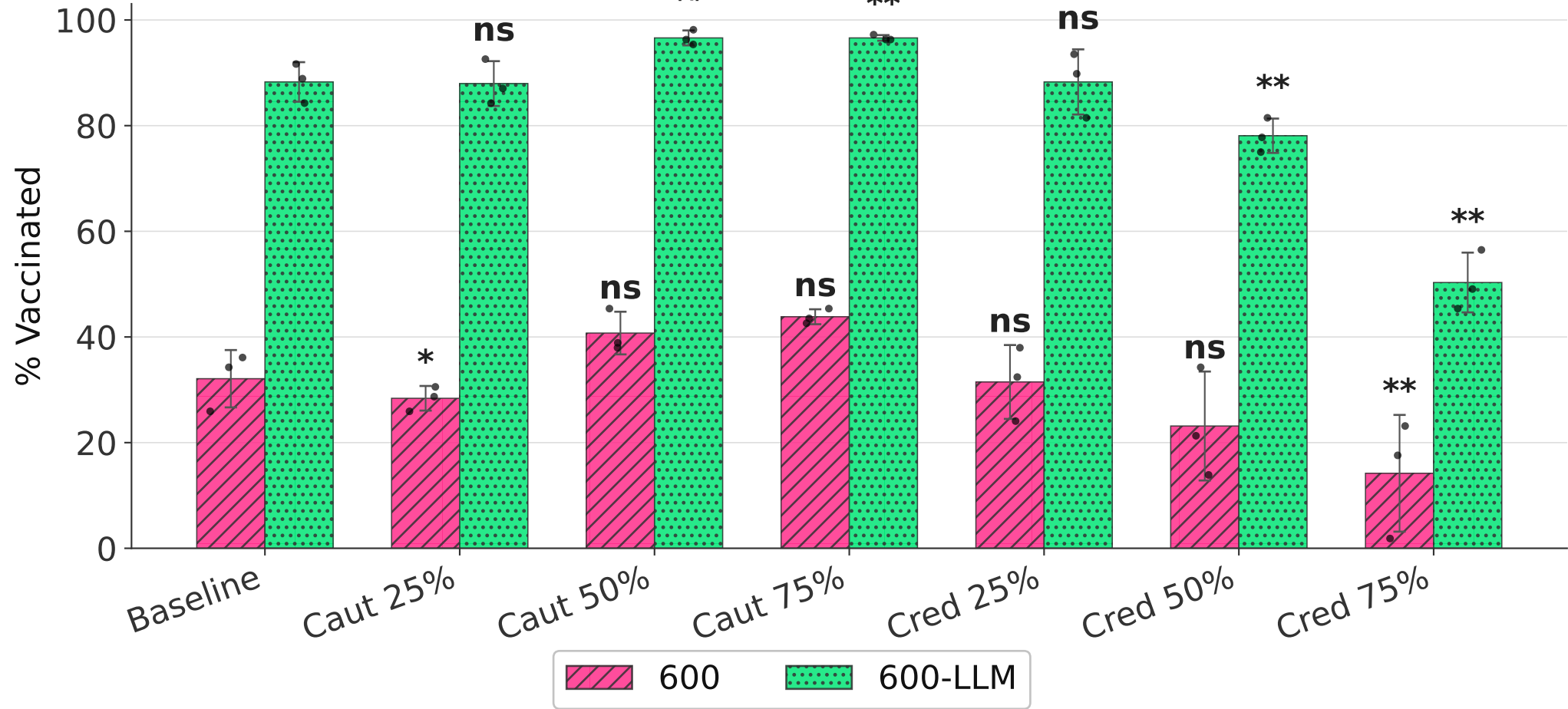
% Vaccinated (of susceptibles) - Thread A (108 susc.) (absolute)
