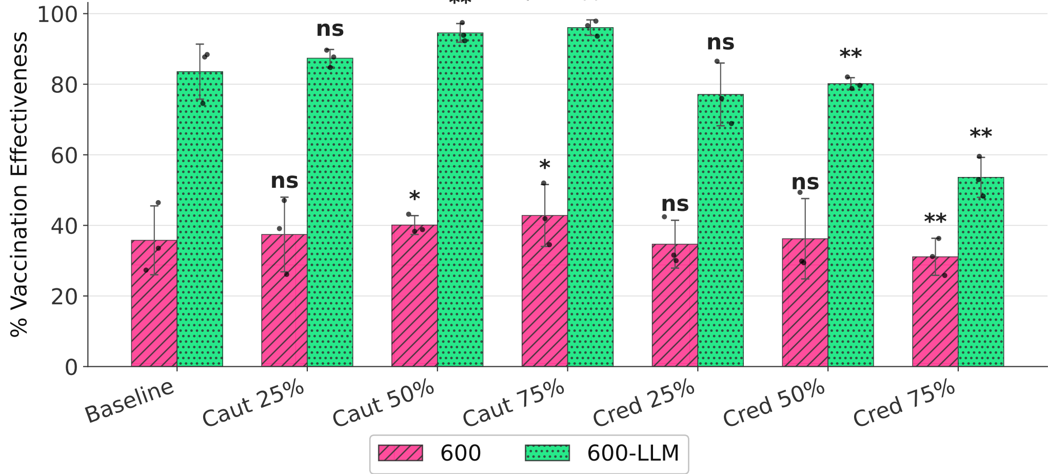
Vaccination Effectiveness (of susceptibles) - Thread B (236 susc.) (absolute)
