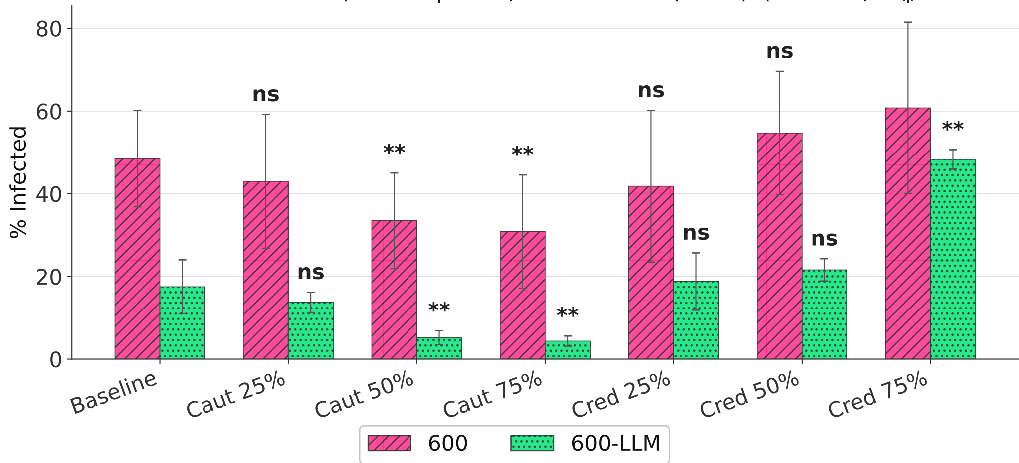
% Infected (of susceptibles) - All threads (mean) (absolute)
