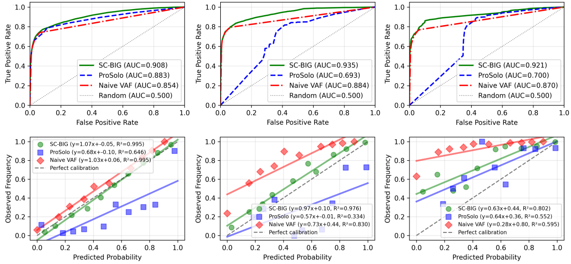
Figure 4: CCF-stratified method comparison. Left column: low CCF stratum ( CCF \in (0, 0.3] ). Middle column: mid CCF stratum ( CCF \in (0.3, 0.7] ). Right column: high CCF stratum ( CCF \in (0.7, 1.0] ). Rows show ROC curves (top) and calibration plots (bottom).
