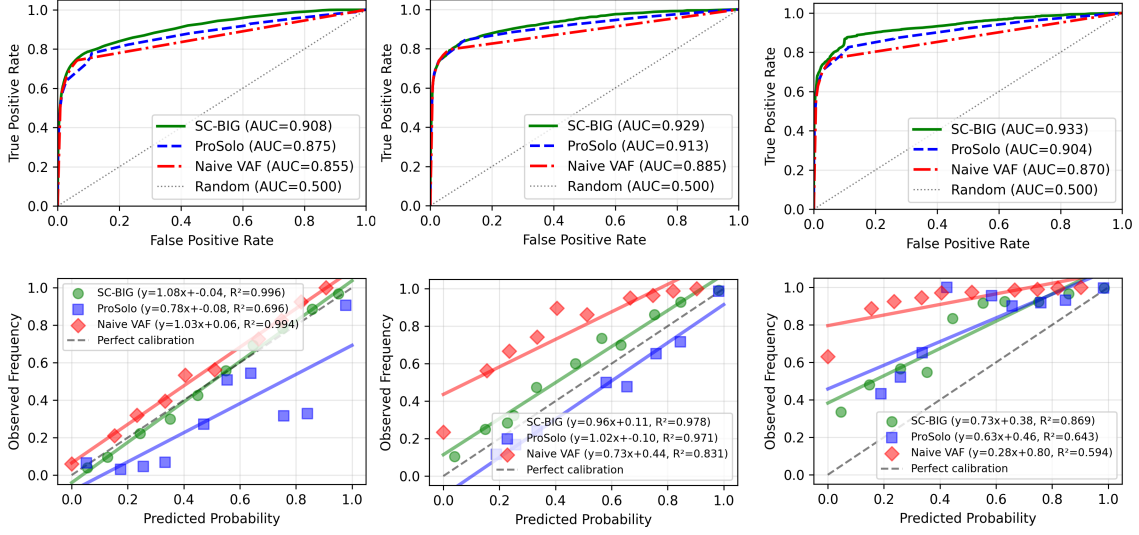
Figure 6: CCF-stratified method comparison for an impure tumor ( \pi = 0.5 ) . Left column: low CCF stratum ( CCF \in (0, 0.3] ). Middle column: mid CCF stratum ( CCF \in (0.3, 0.7] ). Right column: high CCF stratum ( CCF \in (0.7, 1.0] ). Rows show ROC curves (top) and calibration plots (bottom).
