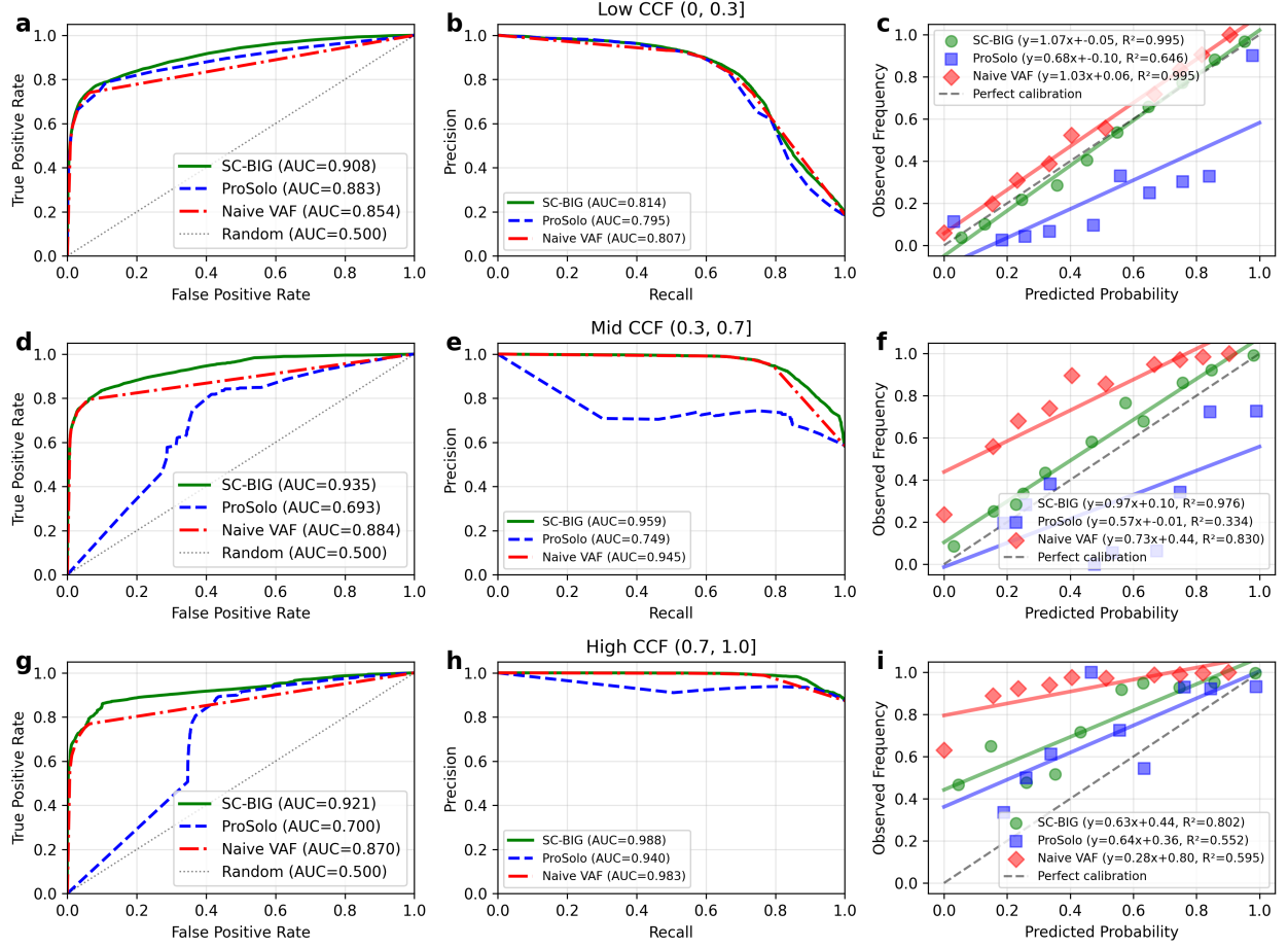
Figure 5: CCF-stratified method comparison. Top row (a–c): low CCF stratum ( CCF \in (0, 0.3] ). Middle row (d–f): mid CCF stratum ( CCF \in (0.3, 0.7] ). Bottom row (g–i): high CCF stratum ( CCF \in (0.7, 1.0] ). Columns show ROC curves (left), PR curves (center), and calibration plots (right).
