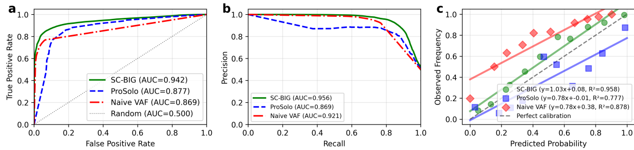
Figure 4: Overall method comparison. (a) ROC curves for SC-BIG, ProSolo, and naive VAF thresholding across all mutations. (b) Precision-recall curves. (c) Calibration plots with linear fits.
