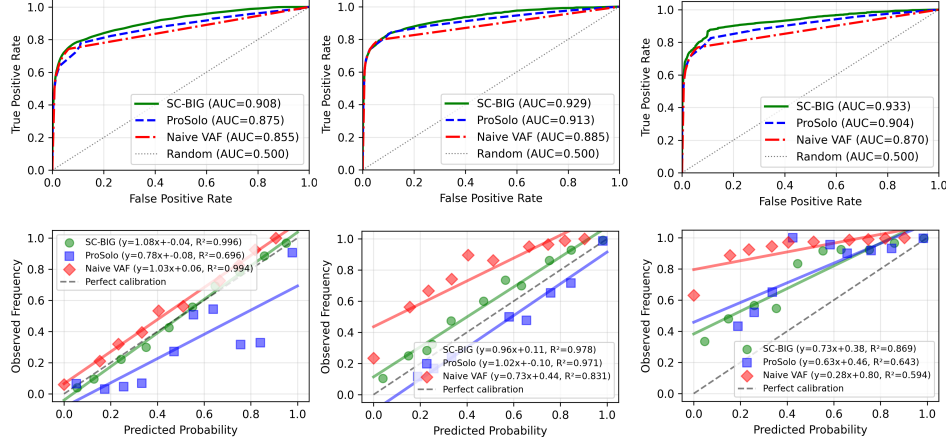
Figure 6: CCF-stratified method comparison for an impure tumor ( \pi = 0.5 ) . Left column: low CCF stratum (CCF \in (0, 0.3] ). Middle column: mid CCF stratum (CCF \in (0.3, 0.7] ). Right column: high CCF stratum (CCF \in (0.7, 1.0] ). Rows show ROC curves (top) and calibration plots (bottom).
