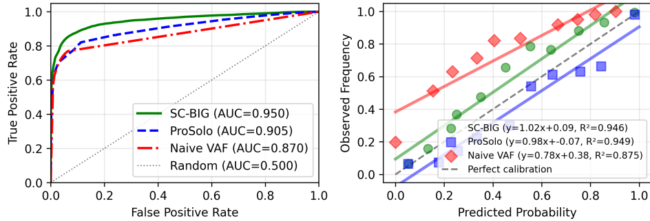
Figure 5: Overall method comparison for an impure tumor ( \pi = 0.5 ). Left: ROC curves for SC-BIG, ProSolo, and naive VAF thresholding across all mutations. Right: Calibration plots with linear fits.
