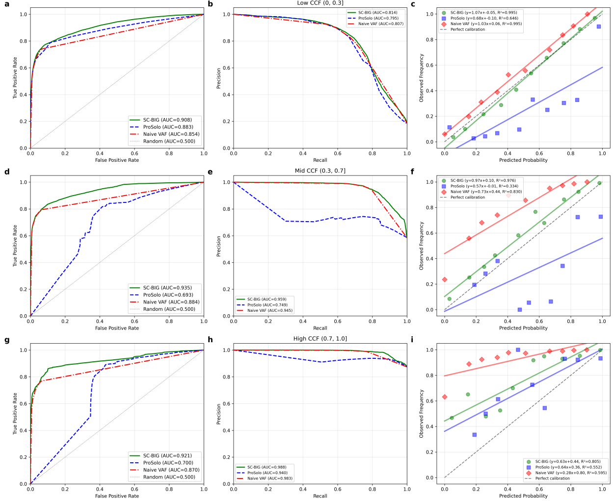
Figure 5: CCF-stratified method comparison. Top row (a–c): low CCF stratum (CCF \in (0, 0.3] ). Middle row (d–f): mid CCF stratum (CCF \in (0.3, 0.7] ). Bottom row (g–i): high CCF stratum (CCF \in (0.7, 1.0] ). Columns show ROC curves (left), PR curves (center), and calibration plots (right).
