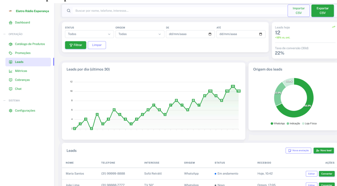
Figura 37 – Leads
