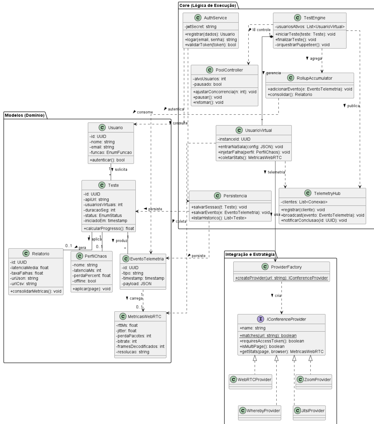
Figura 9: Diagrama de Classes do Stream Sentry
