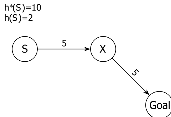
Figure 1: The heuristic h is admissible since it's less to the actual cost to the goal.
