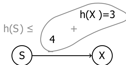
Figure 2: h(s) is consistent since it's less than the cost to transition to the next node, and the heuristic of that next node (X).
