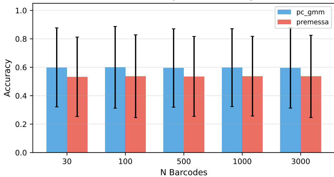
18ch: Accuracy at 80% Coverage
