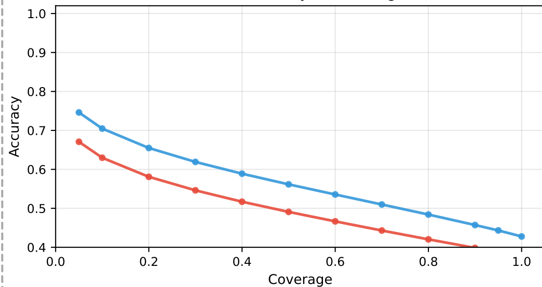
27ch: Accuracy vs Coverage
