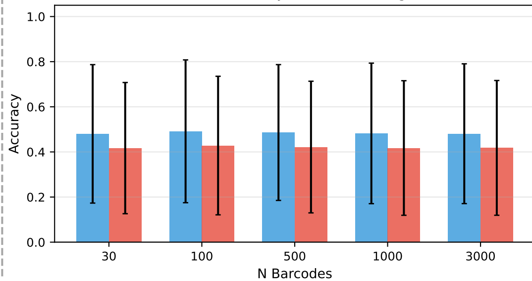
27ch: Accuracy at 80% Coverage
