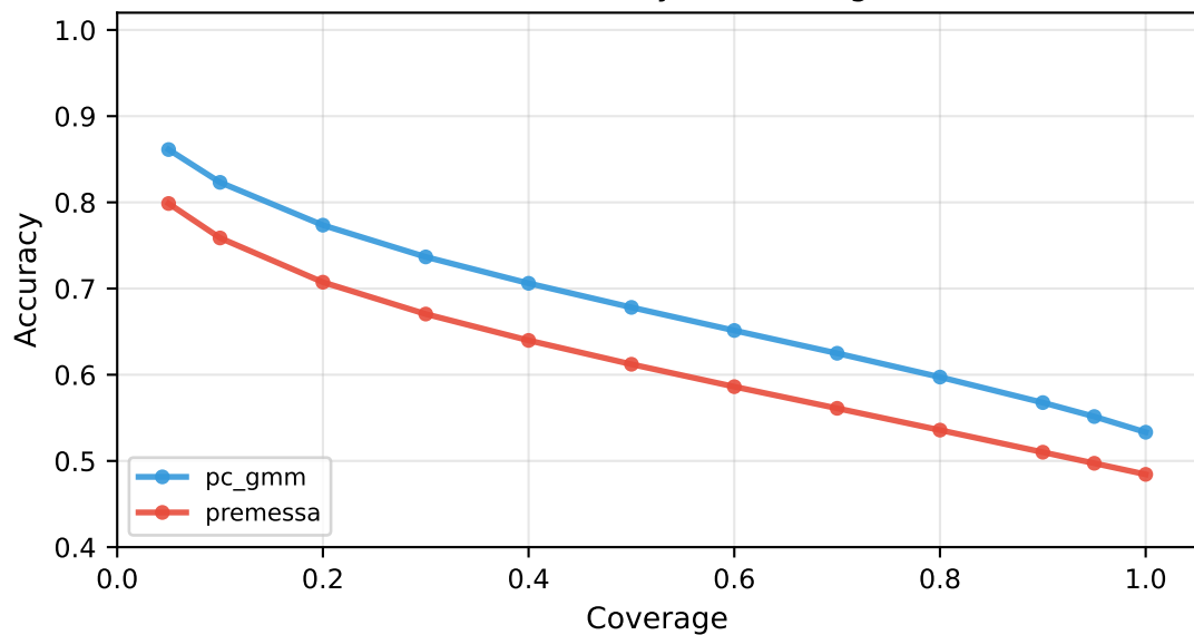
18ch: Accuracy vs Coverage
