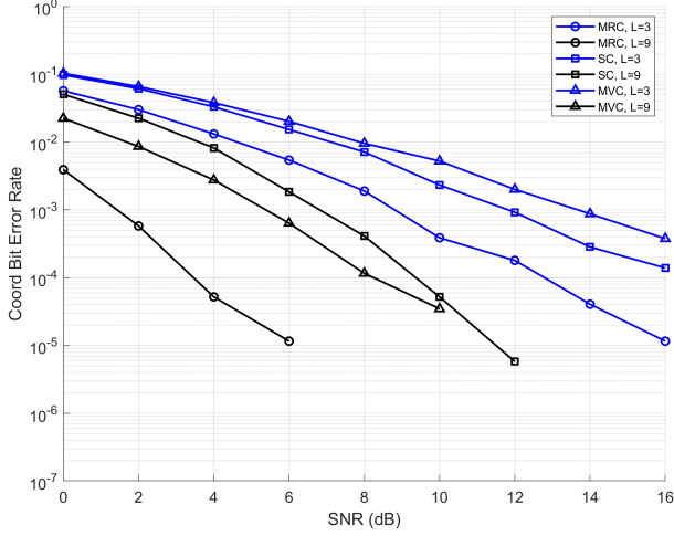
Fig. 3. The BER performance of the coordinates under different merging strategies.
