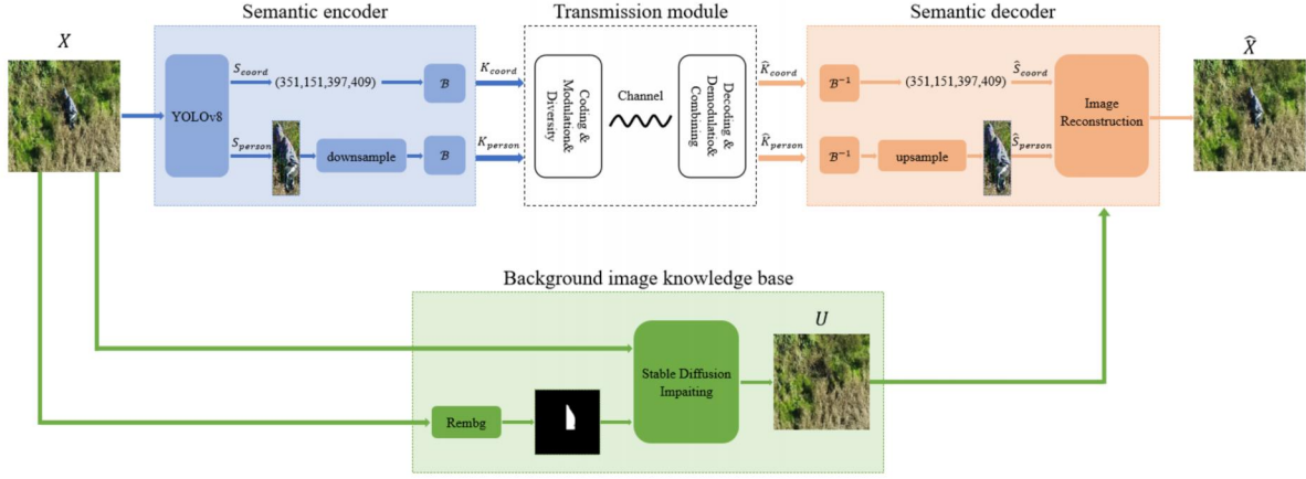
Fig. 1. The proposed semantic communication system for wilderness search and rescue scenarios.
