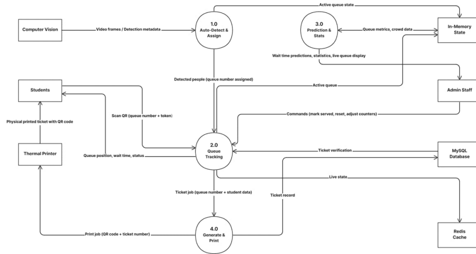
Figure 2.2: Data Flow Diagram 0
