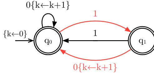
Figure 7: Constructed cDFA, K = \{1, 3\}
