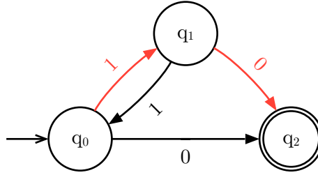
Figure 6: Intermediate finite automaton, K = \{1, 3\}
