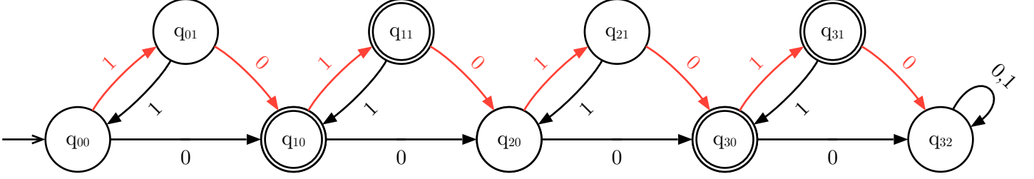
Figure 8: Equivalent DFA
