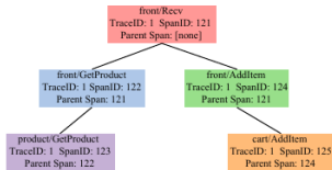
Figure 2: The trace coverage tree of Fig. 1
