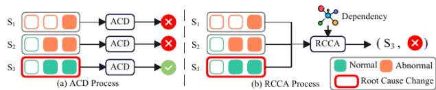
Fig. 2. Comparison between abnormal change detection (ACD) and root cause change analysis (RCCA).
