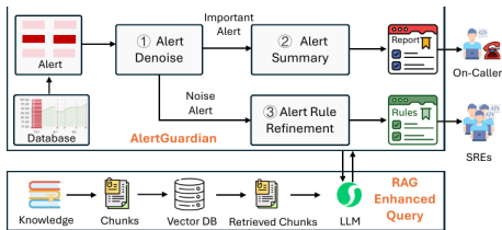
Fig. 9: Overview of AlertGuardian in Company-X.
