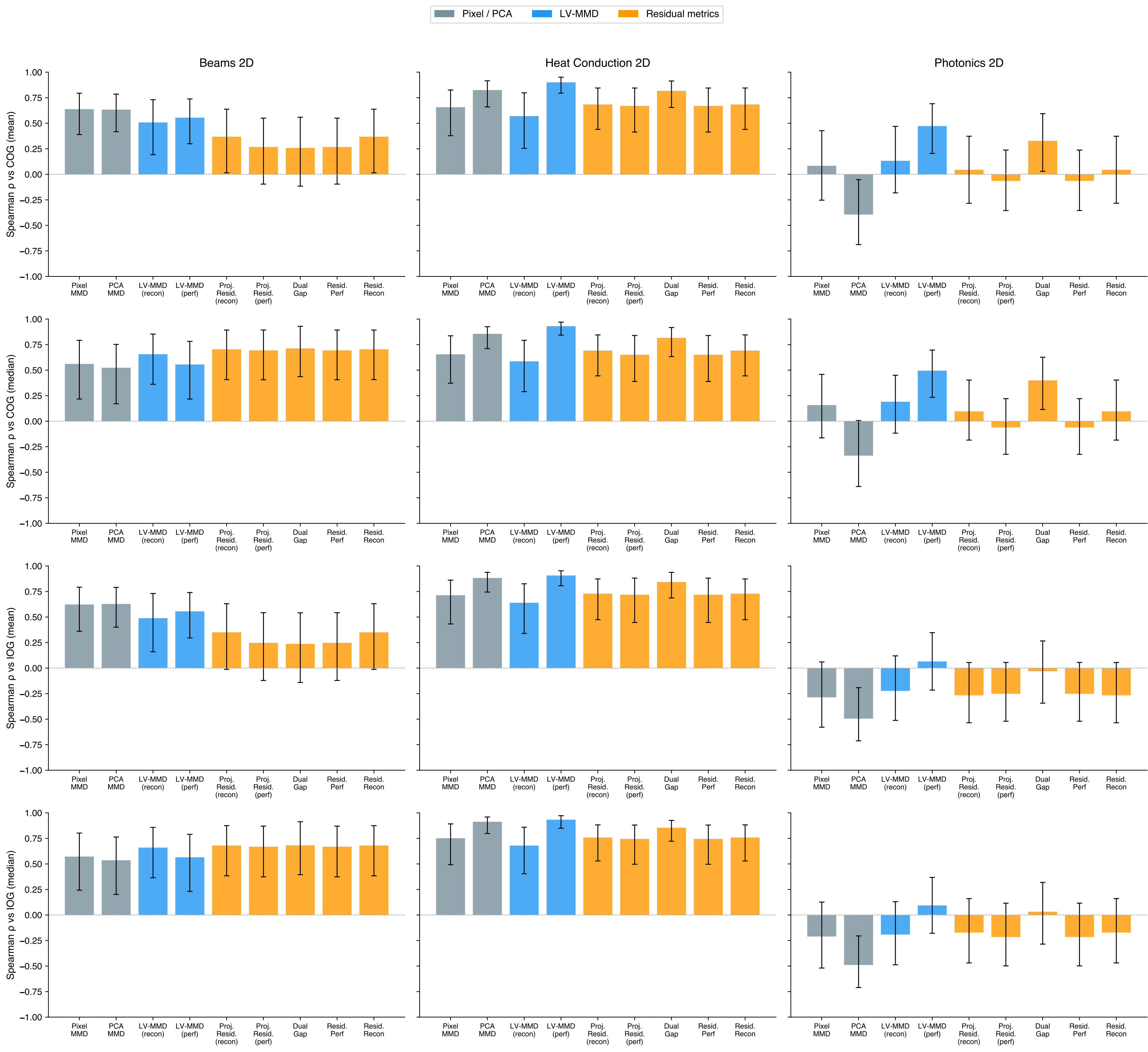
Extended Ablation Ladder: Correlation with Optimality Gaps (95% bootstrap CI)
