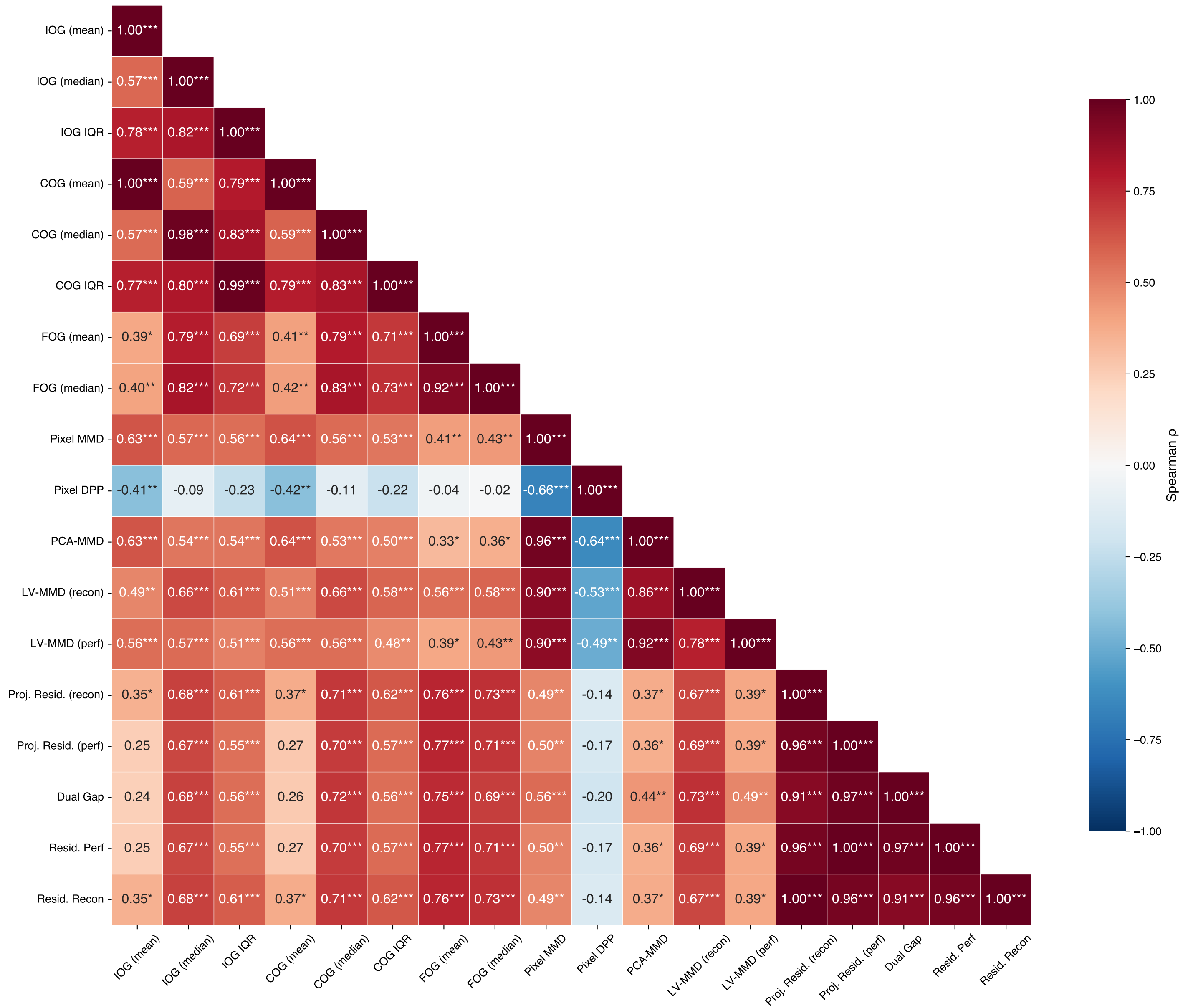
Cross-Metric Correlation — Beams 2D
