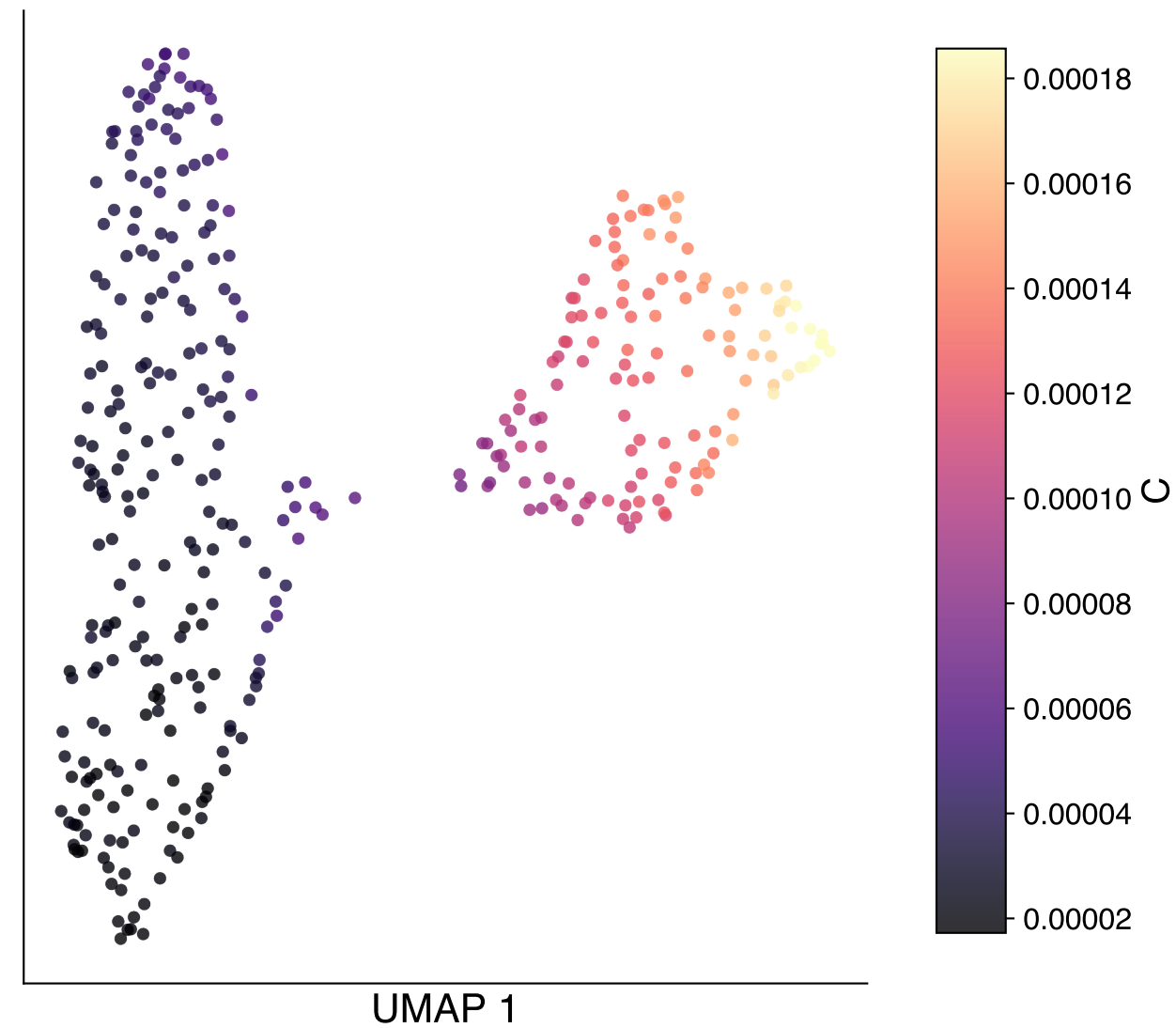
LVAE (perf NMSE=0.005) 9 active dims
