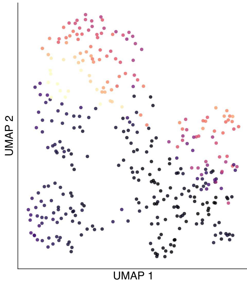
Pixel Space (10,000 dims)
