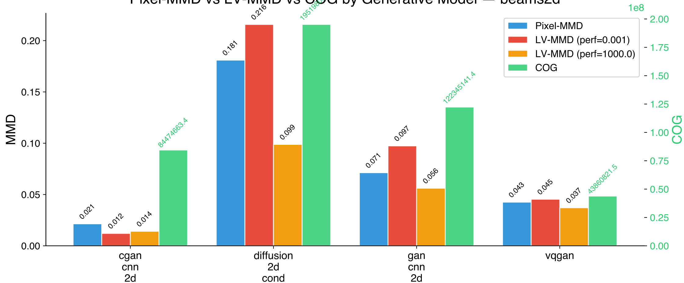
Pixel-MMD vs LV-MMD vs COG by Generative Model — beams2d
