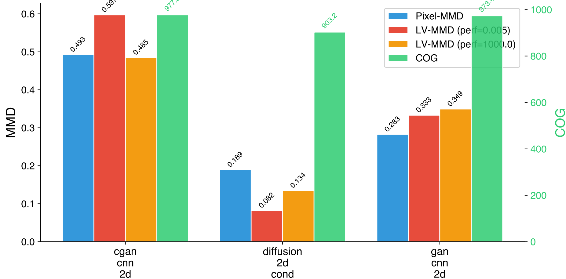
Pixel-MMD vs LV-MMD vs COG by Generative Model — photonics2d
