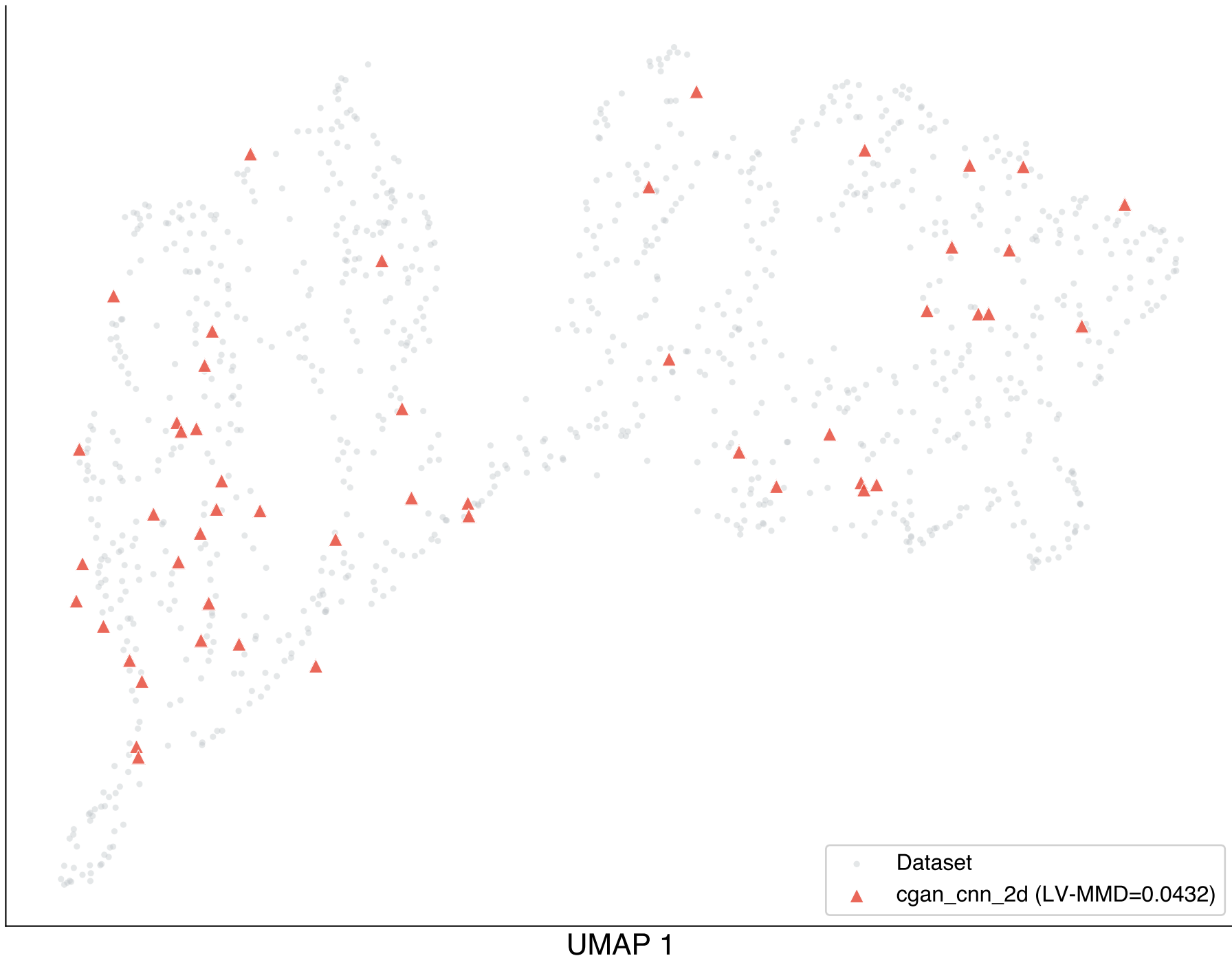
Generated Samples in LVAE Latent Space — beams2d
