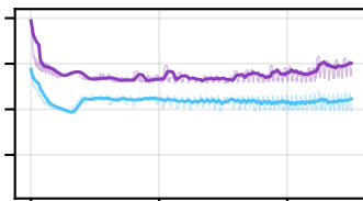
PAL: f(\tilde{y}^{(1)})
