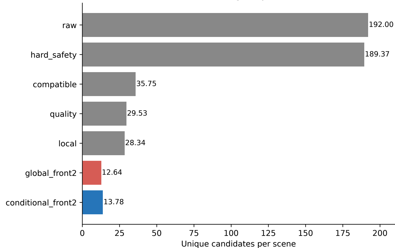
Full-1000 eligibility funnel
