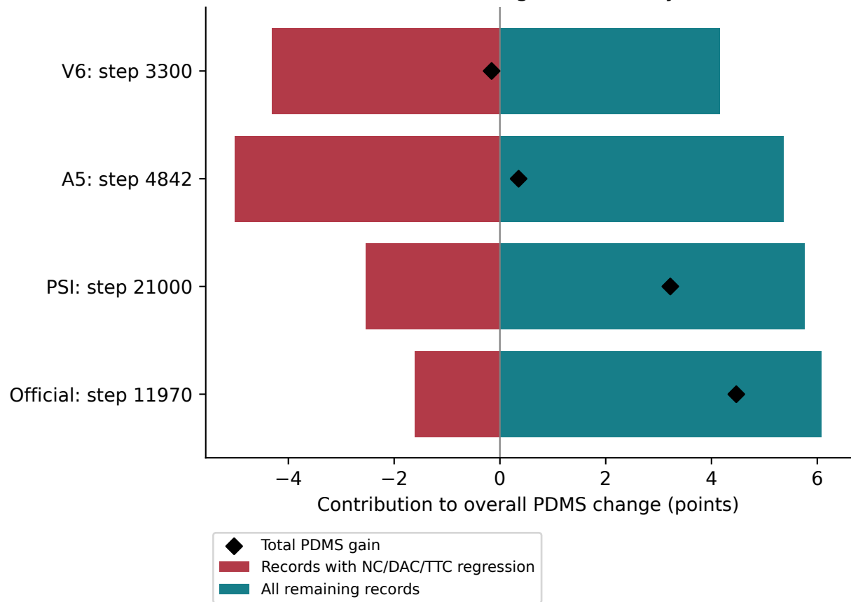
Exact accounting of the safety tail
