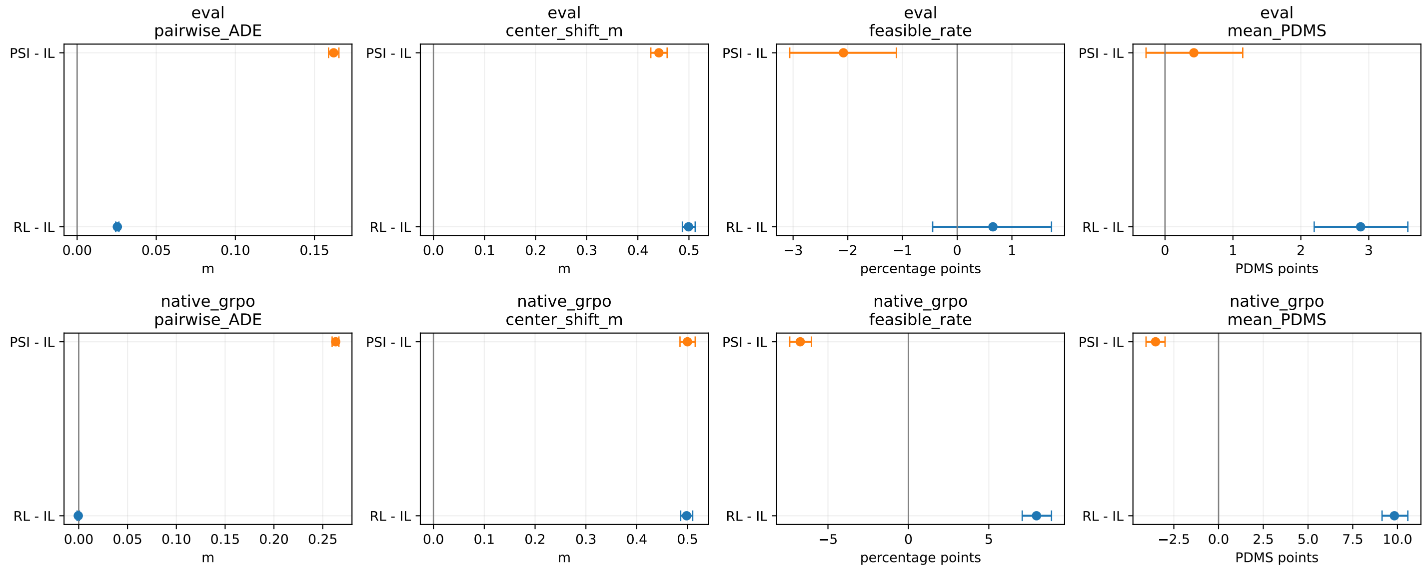
Full 1000 scenes: paired effects and 95% scene-bootstrap CI
