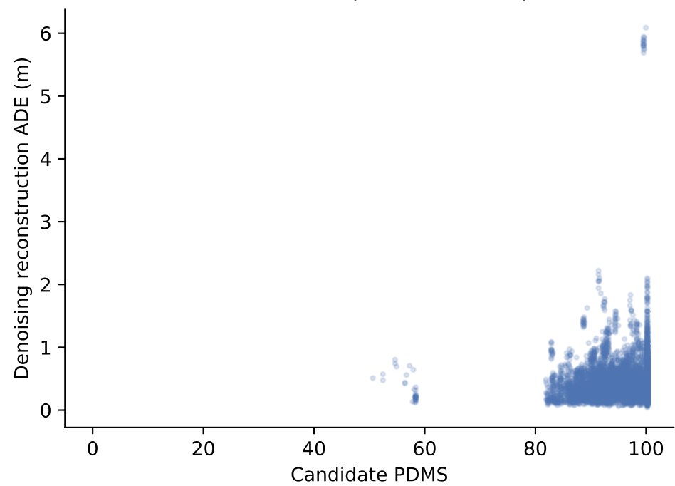
GT-distance (n=500 scenes)
