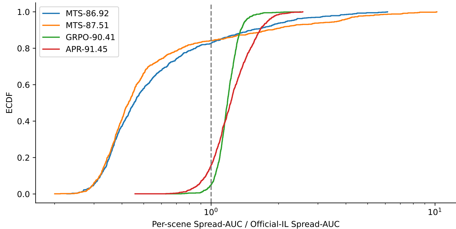
Observed checkpoint compression and expansion; V1 rollouts reused
