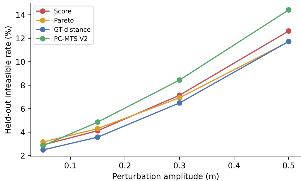
contrastive
