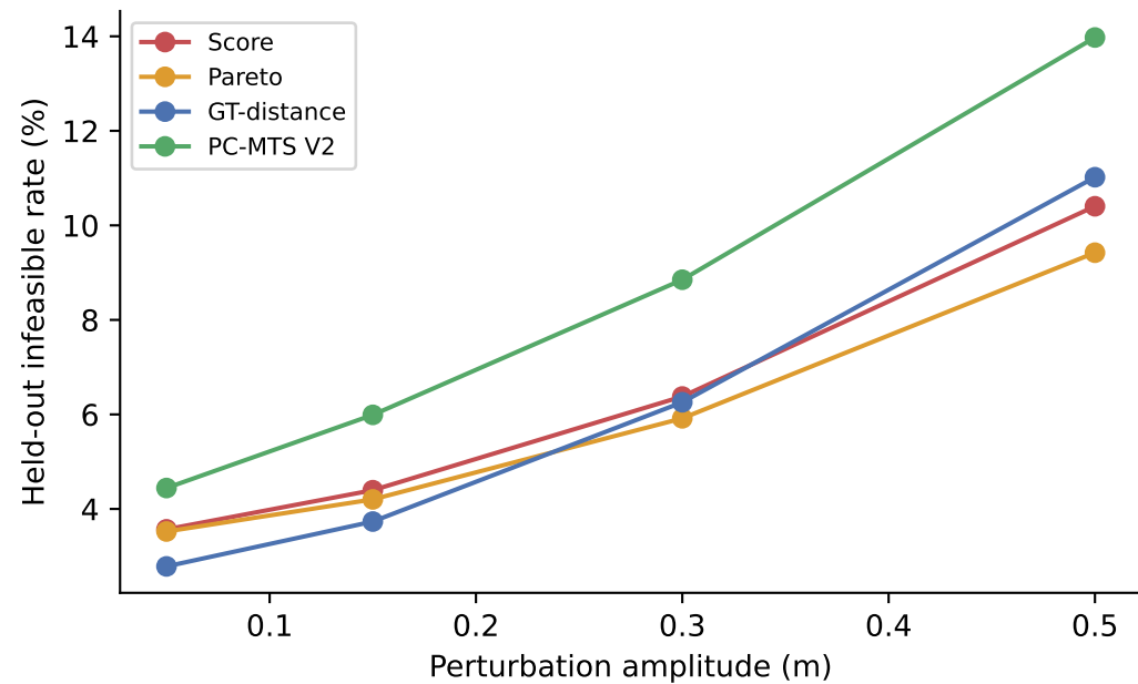
full1000
