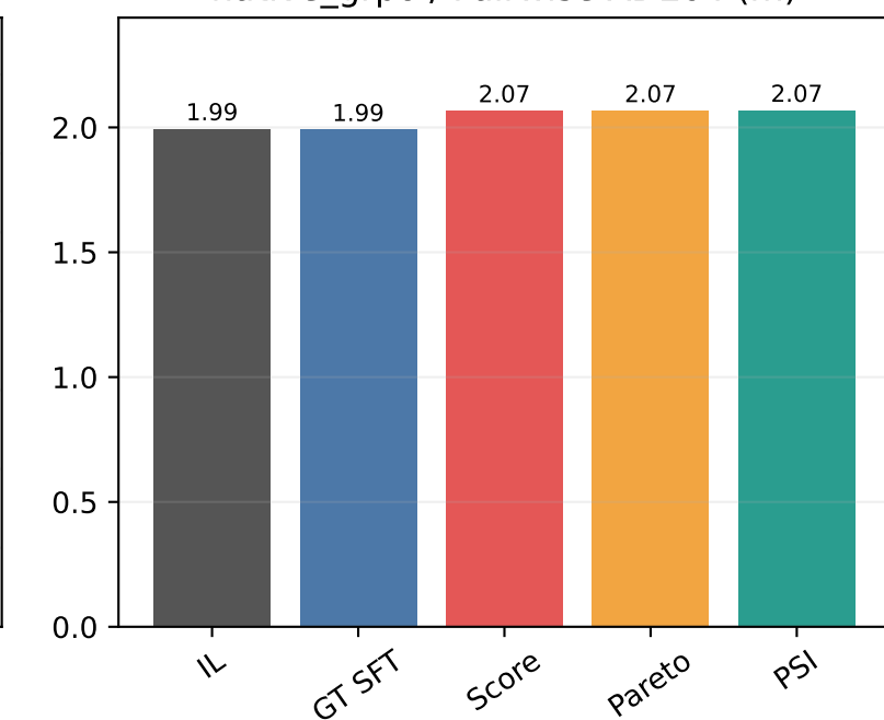
native_grpo / Pairwise ADE64 (m)
