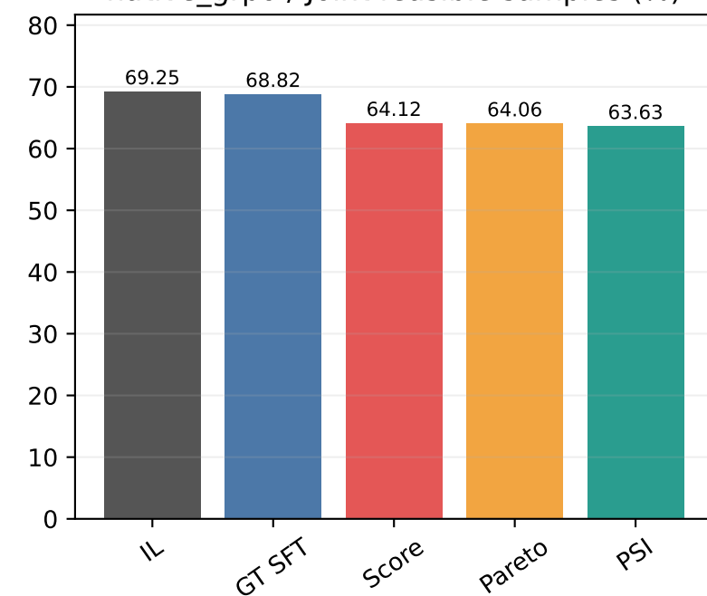
native_grpo / Joint feasible samples (%)
