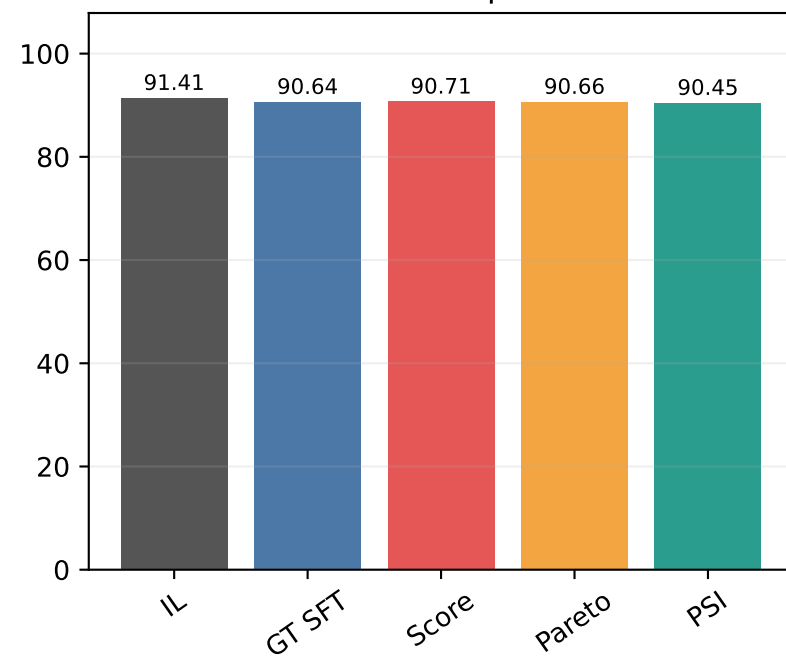
native_grpo / Mean sampled PDMS
