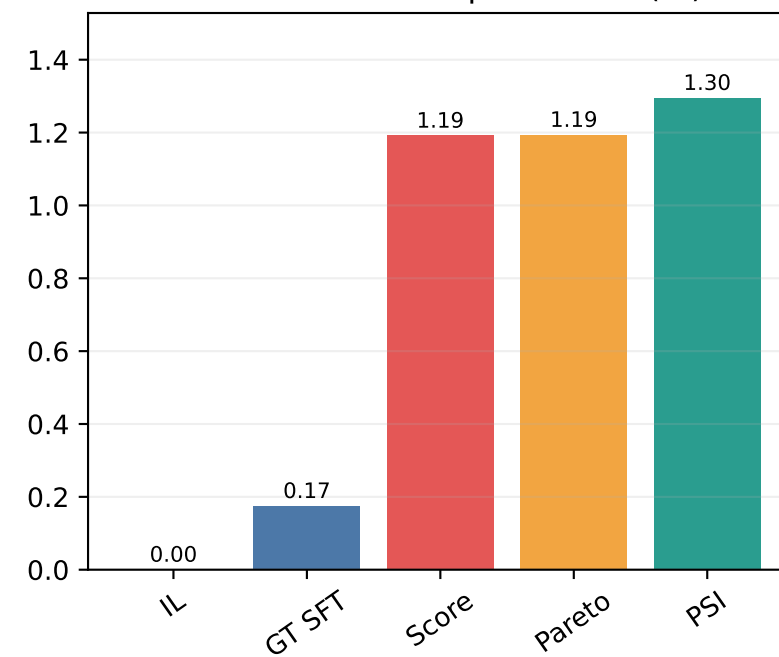
native_grpo / Centroid displacement (m)
