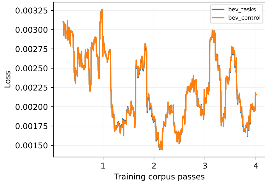
100-step mean original DiT ego FM loss
