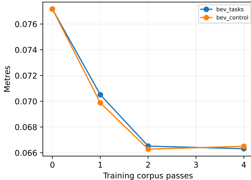
Fixed train64 original DiT trajectory ADE
