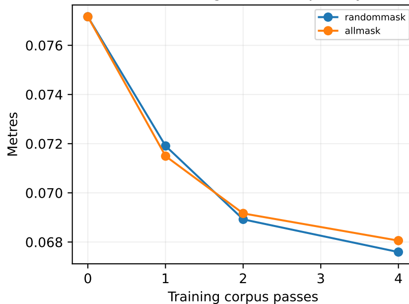
Fixed train64 original DiT trajectory ADE
