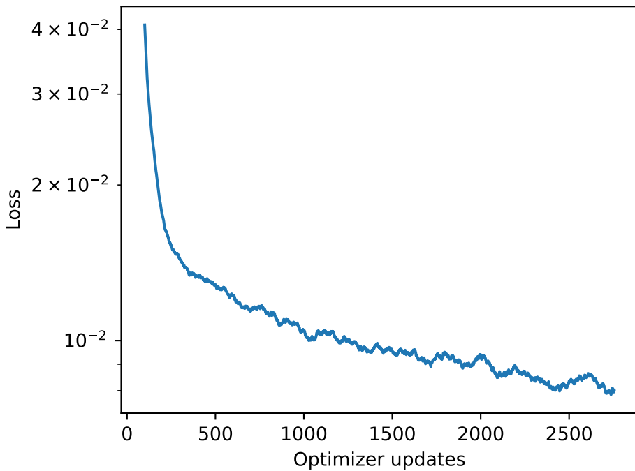
Train Smooth L1 (100-step mean)
