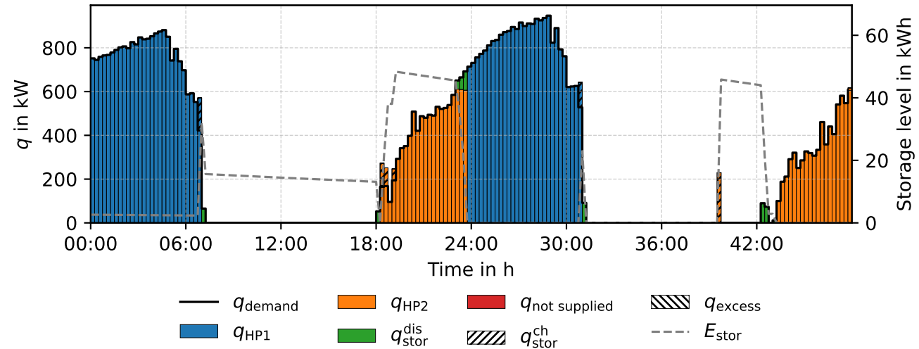
Heat balance - RP rp01 (CR)
