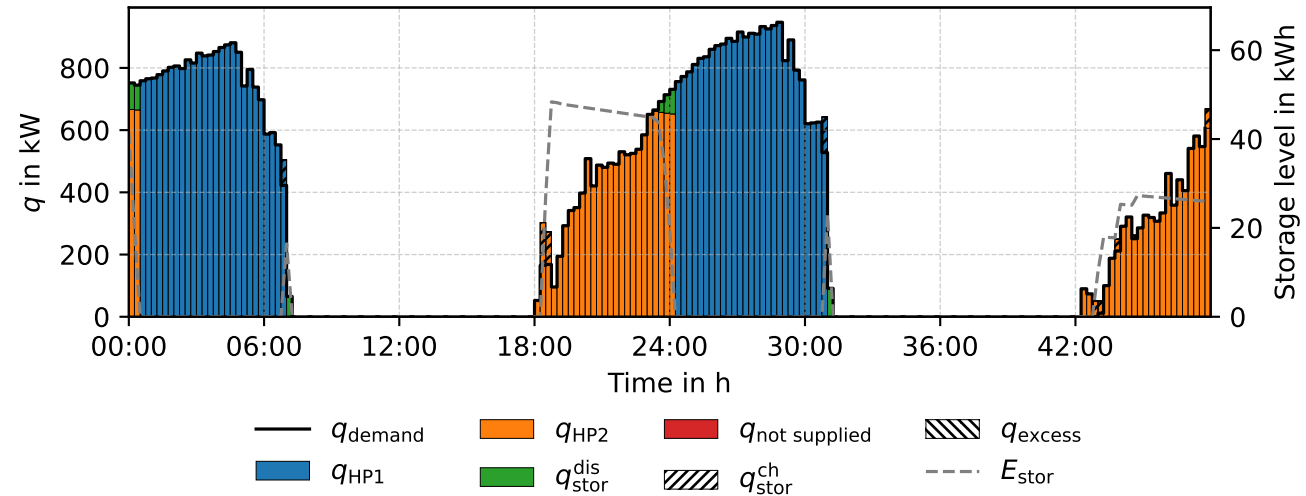
Heat balance – RP rp01 (PWL)
