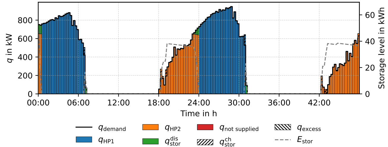
Heat balance – RP rp01 (PWLR)
