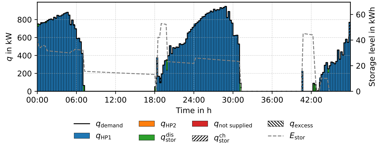
Heat balance - RP rp01 (UC)
